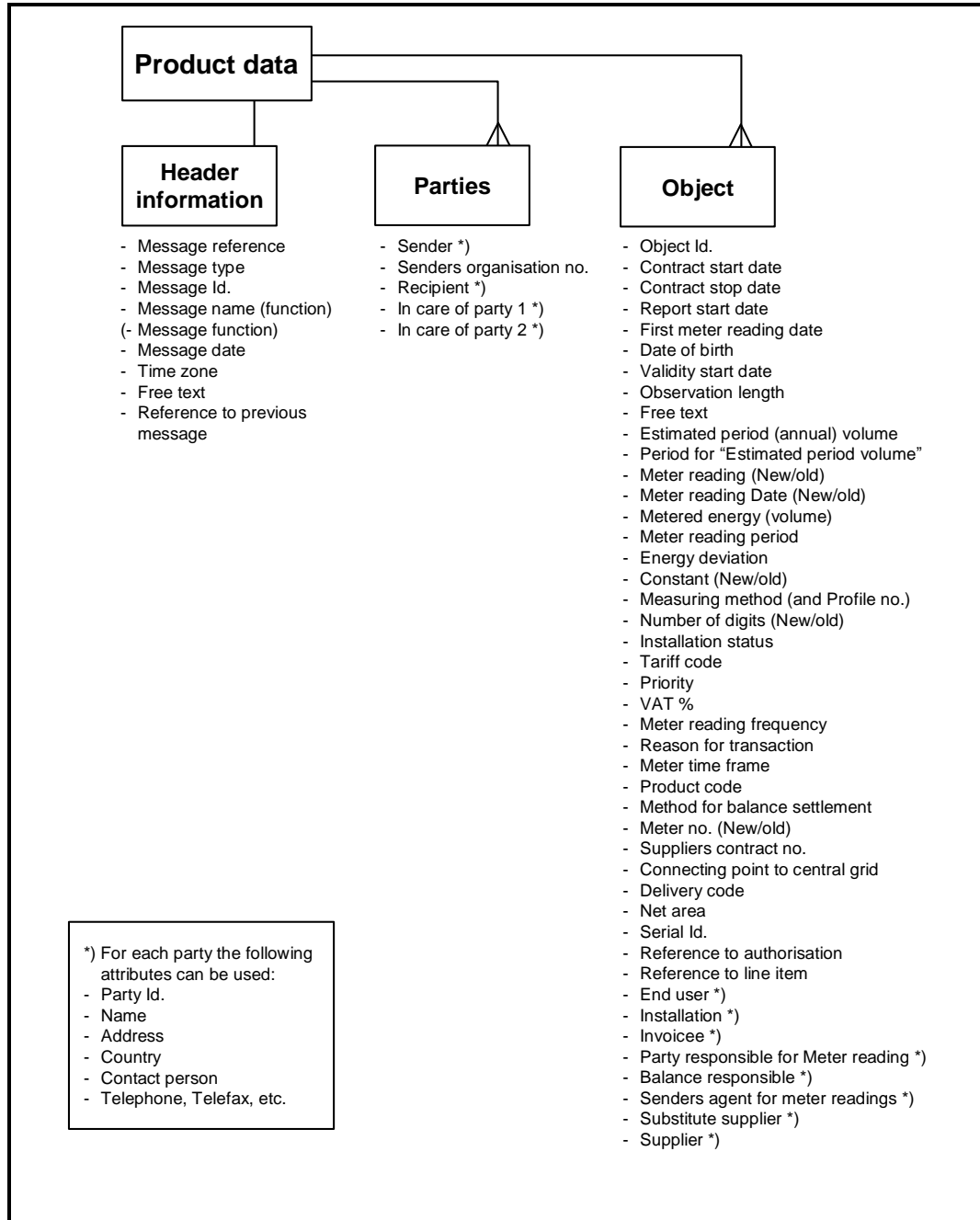
Figure 1 Data model for the Product data message
